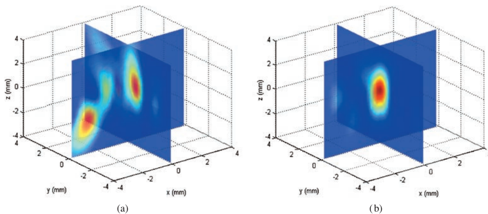
Figure 7. A third example of focusing using case 2 after projecting the planar data over a 3D volume. Field intensities are shown (a) before phase correction and (b) after non-invasive correction.
