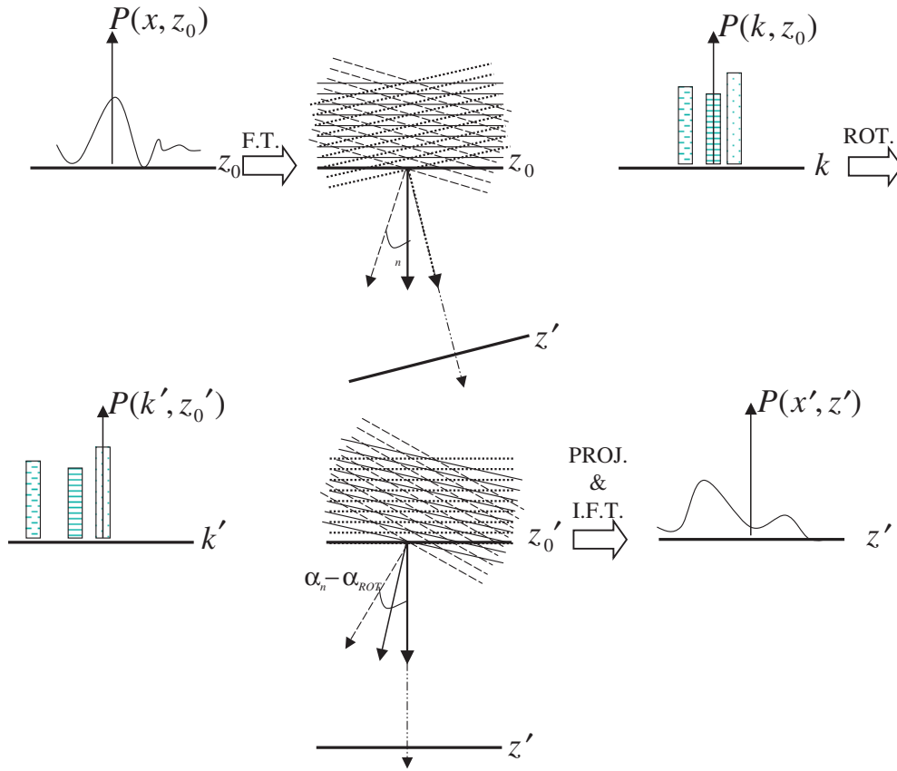
Figure 1. Illustration of the projection method. The field initially at the plane perpendicular to z_0 is rotated and projected to a new plane perpendicular to z' .
