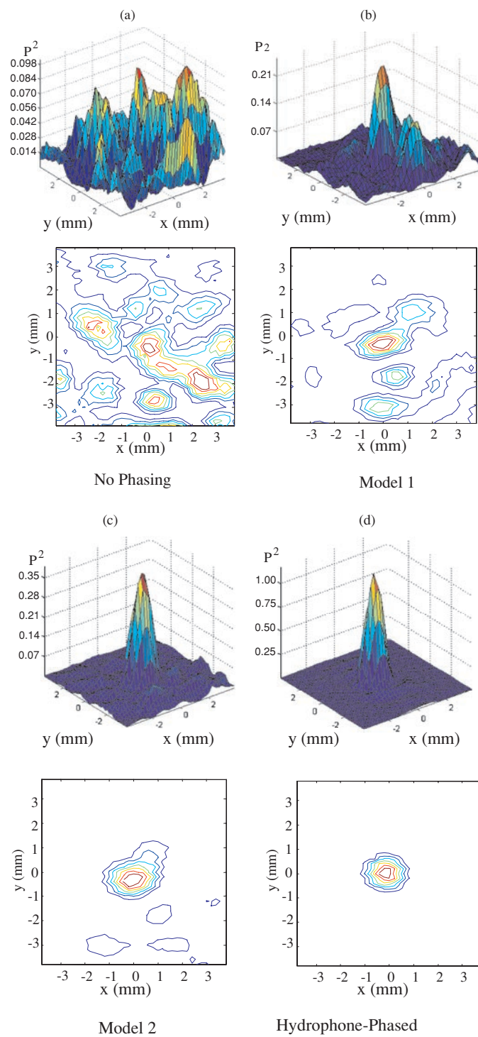
Figure 5. Relative pressure squared near the array's geometric centre: (a) without phase correction, (b) with non-invasive correction using case 1, (c) with non-invasive correction using case 2 and (d) with a hydrophone-assisted focus.
