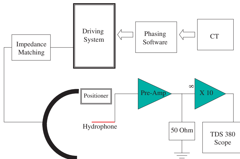
Figure 4. The experimental set-up.
