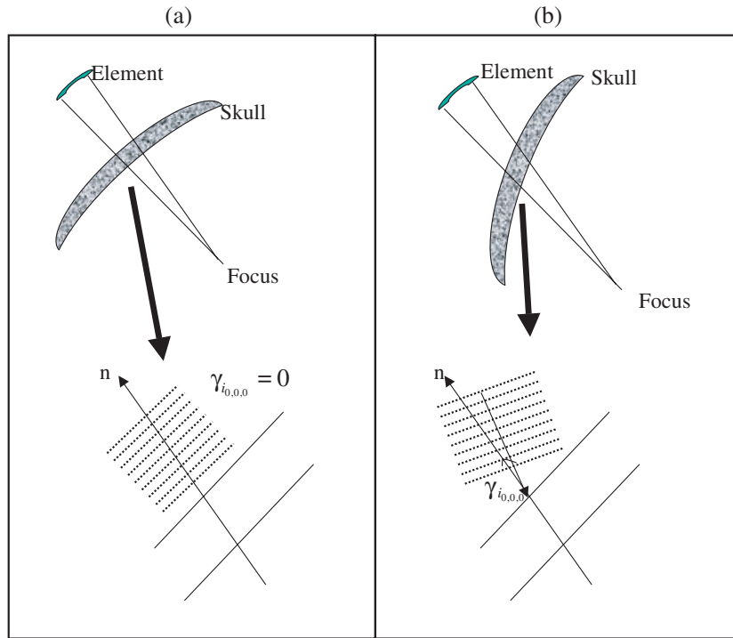
Figure 2. The two propagation cases studied. Case 1 (a) assumes that the ultrasound is incident upon the skull. Case 2 (b) calculates the orientation between the field and the skull surface.
