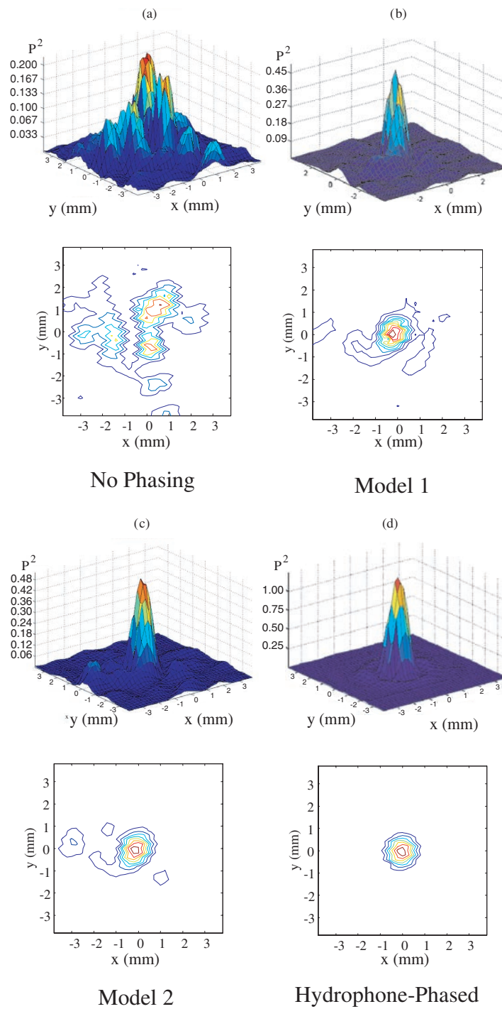
Figure 6. A second example of the focus: (a) without phase correction, (b) with non-invasive correction using case 1, (c) with non-invasive correction using case 2 and (d) with a hydrophone-assisted focus.
